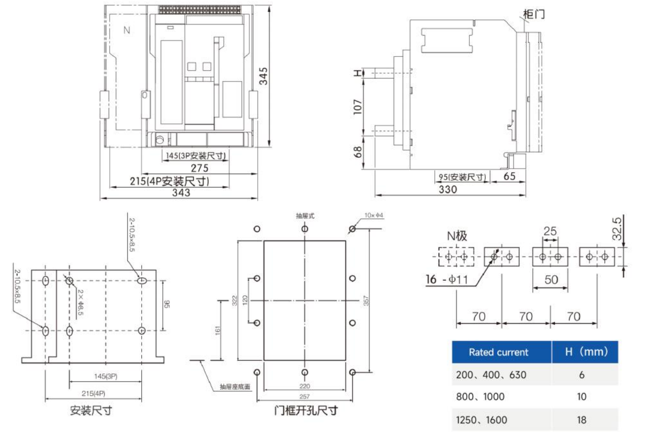
CQW2-1600 Series Drawout Type Installation Dimensions (Unit: mm)
