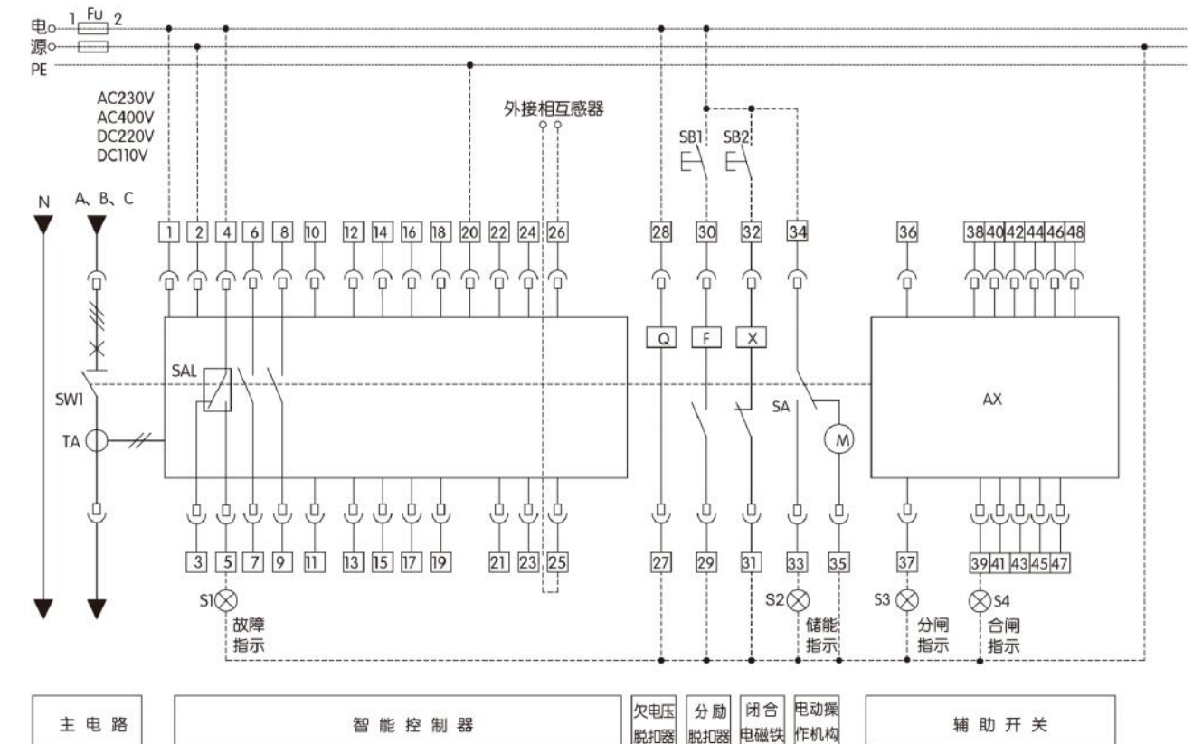
Wiring diagram of secondary circuit for SW1-1600-6300 circuit breakers equipped with L/M type intelligent controllers (auxiliary switch default configuration: 4 changeover contacts)
