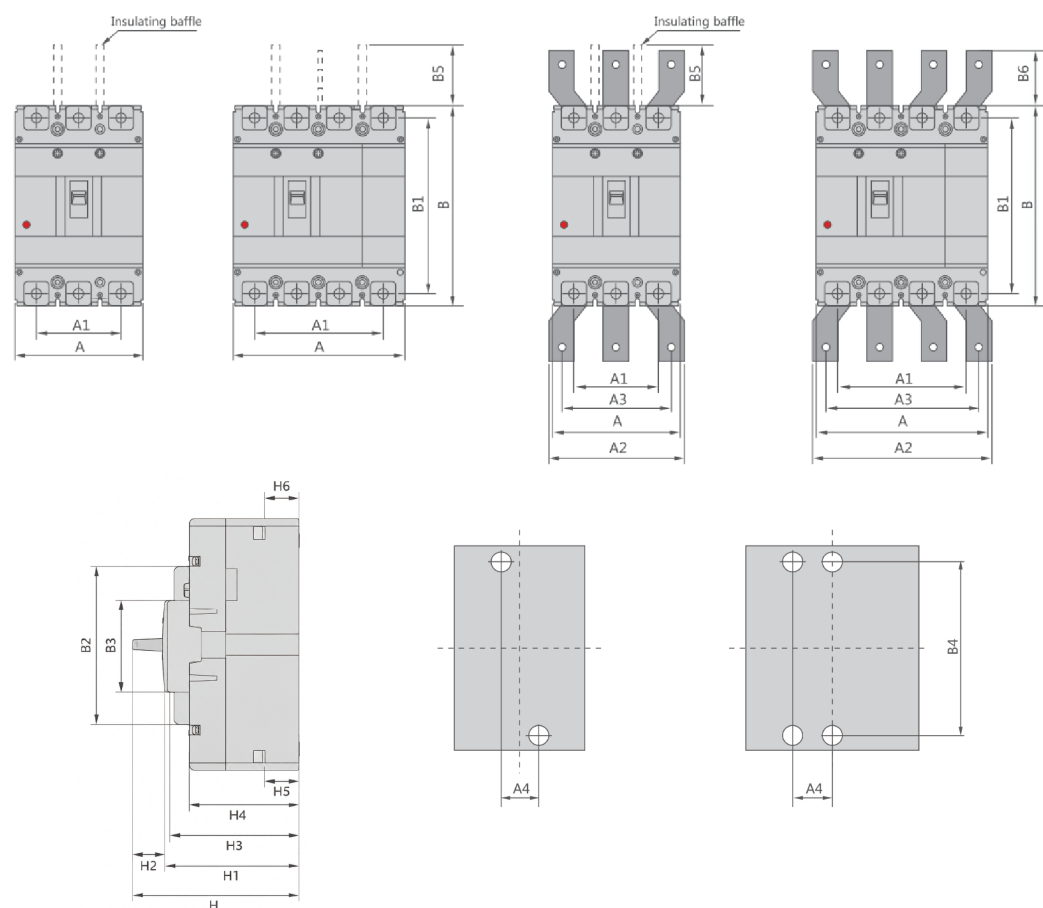
CQM6-125~1250 Outline and Installation Dimensions(mm)
